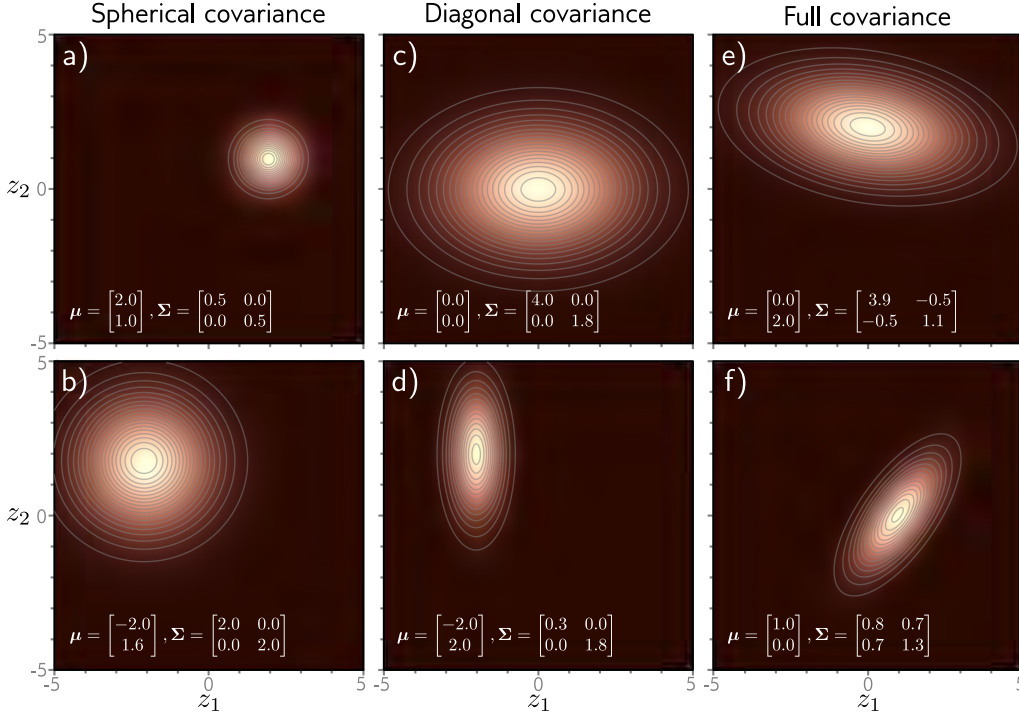
Figure C.4 Bivariate normal distribution. a–b) When the covariance matrix is a multiple of the identity matrix, the isocontours are circles, and we refer to this as spherical covariance. c–d) When the covariance is an arbitrary diagonal matrix, the isocontours are axis-aligned ellipses, and we refer to this as diagonal covariance. e–f) When the covariance is an arbitrary symmetric positive definite matrix, the isocontours are general ellipses, and we refer to this as full covariance.
