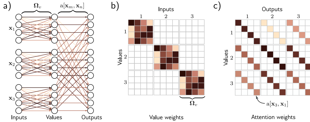
Figure 12.2 Self-attention for N=3 inputs \mathbf{x}_n , each with dimension D=4 . a) Each input \mathbf{x}_n is operated on independently by the same weights \Omega_v (same color equals same weight) and biases \beta_v (not shown) to form the values \beta_v + \Omega_v \mathbf{x}_n . Each output is a linear combination of the values, with the attention weight a[\mathbf{x}_m, \mathbf{x}_n] defining the contribution of the m^{\text{th}} value to the n^{\text{th}} output. b) Matrix showing block sparsity of linear transformation \Omega_v between inputs and values. c) Matrix showing sparsity of attention weights relating values and outputs.
