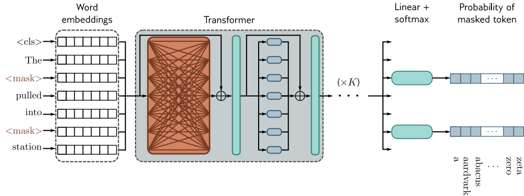
Figure 12.10 Pre-training for BERT-like encoder. The input tokens (and a special <cls> token denoting the start of the sequence) are converted to word embeddings. Here, these are represented as rows rather than columns, so the box labeled “word embeddings” is \mathbf{X}^T . These embeddings are passed through a series of transformer layers (orange connections indicate that every token attends to every other token in these layers) to create a set of output embeddings. A small fraction of the input tokens are randomly replaced with a generic <mask> token. In pre-training, the goal is to predict the missing word from the associated output embedding. To this end, the outputs corresponding to the masked tokens are passed through softmax functions, and a multiclass classification loss (section 5.24) is applied to each. This task has the advantage that it uses both the left and right context to predict the missing word but has the disadvantage that it does not make efficient use of data; here, seven tokens need to be processed to add two terms to the loss function.
